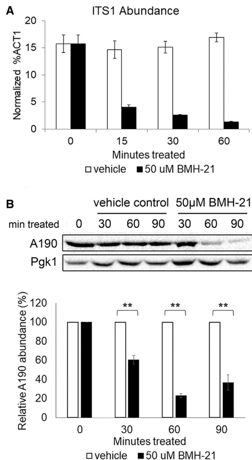
Figure 5. BMH-21 Effect on Pol I Is Conserved in Yeast
