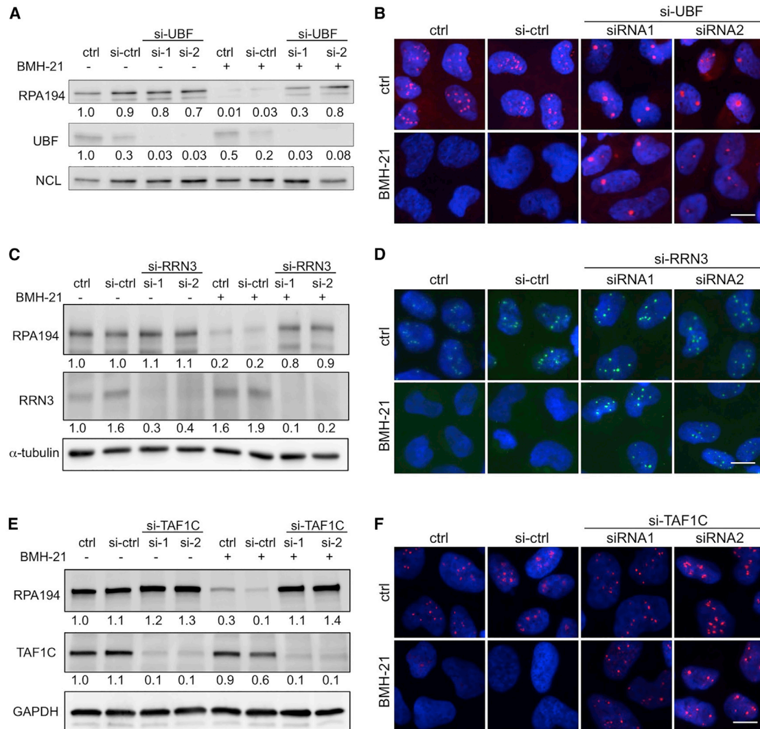
Figure 2. Depletion of the Preinitiation Factors Rescues RPA194 Degradation by BMH-21
