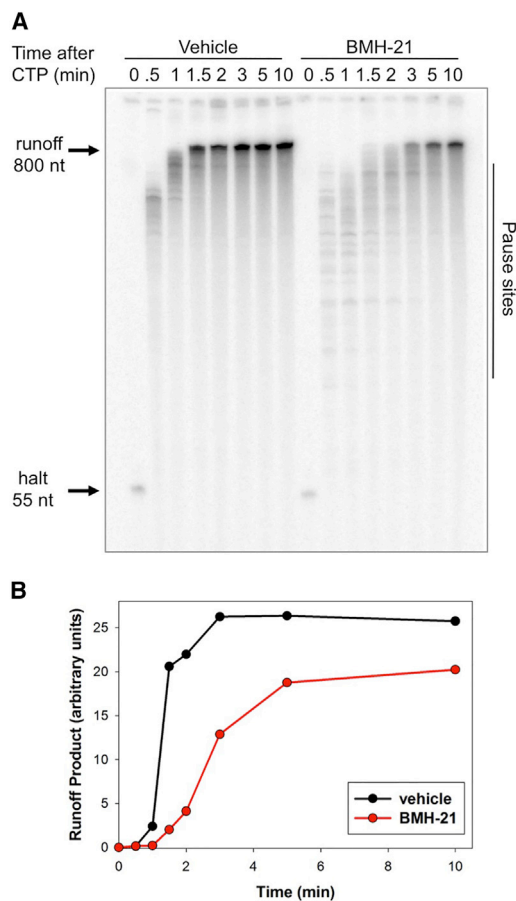
Figure 7. BMH-21 Directly Inhibits Pol I Transcription Elongation
