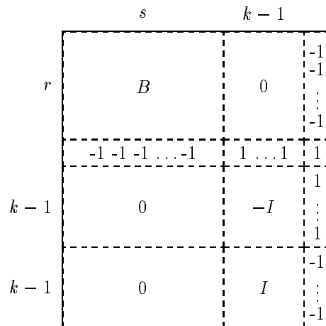
Figure 1: Matrix C .
