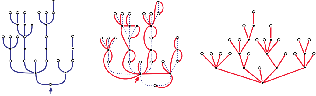
Figure 6: Illustration of the Janson & Stefansson transformation.
