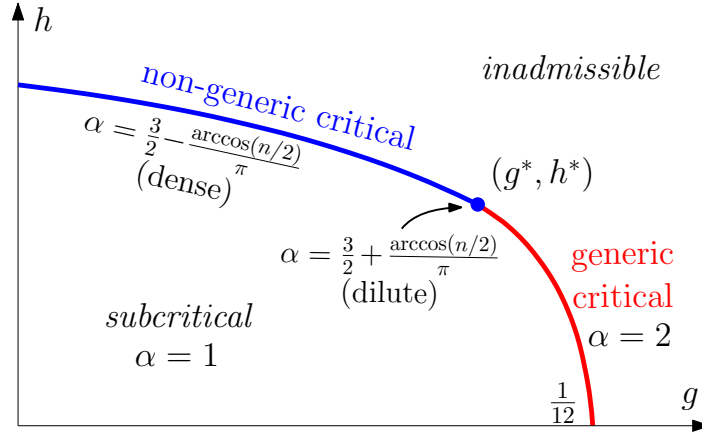
Figure 2: Phase diagram of the loop-decorated quadrangulation model [13, 16] for a given value of n \in (0, 2) (the diagram is qualitatively the same for all such n ). For every admissible set of parameters (n; g, h) , the asymptotic form (3) holds. The different phases are characterized by different values of the exponent \alpha . The critical line separates the sub-critical region (below) and the inadmissible region (above).
