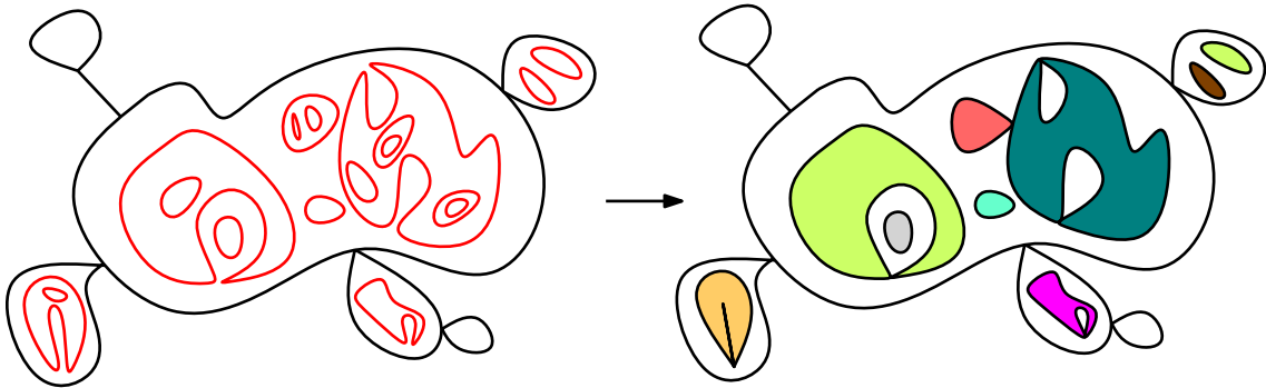
Figure 4: Illustration of the gasket decomposition. Notice that after removing the outer-most loops and their interiors, the holes in the gasket may be non-simple faces. See also [13, Fig. 4]
