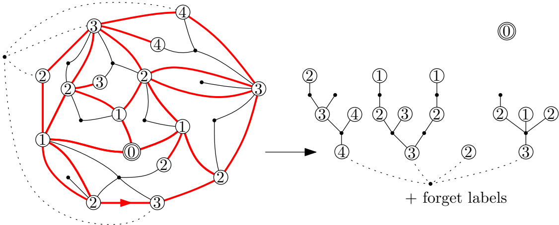
Figure 5: Illustration of the construction of a forest of p mobiles from a pointed bipartite planar map with a boundary of perimeter 2p . The first mobile in the forest is not specified by the map and is chosen uniformly at random among all the mobiles.
