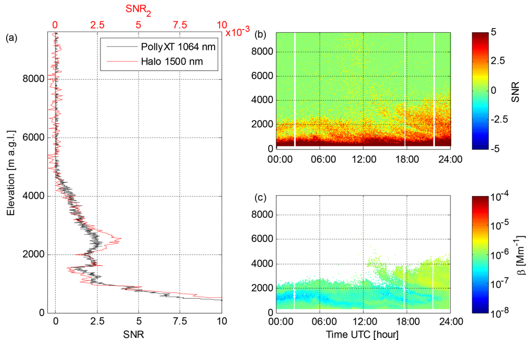
Figure 9. (a) Vertical profiles of SNR from PollyXT at 1064 nm wavelength and \text{SNR}_2 from lidar 53 at Finokalia on 8 July 2014. Both profiles are obtained at 21:00 UTC; the integration time of the lidar 53 profile is 350 s, and the integration time of the PollyXT profile is 360 s. (b) Time series of PollyXT SNR at 1064 nm wavelength with 360 s integration time at Finokalia on 8 July 2014. (c) Time series of PollyXT attenuated backscatter at 1064 nm wavelength with 360 s integration time at Finokalia on 8 July 2014.
