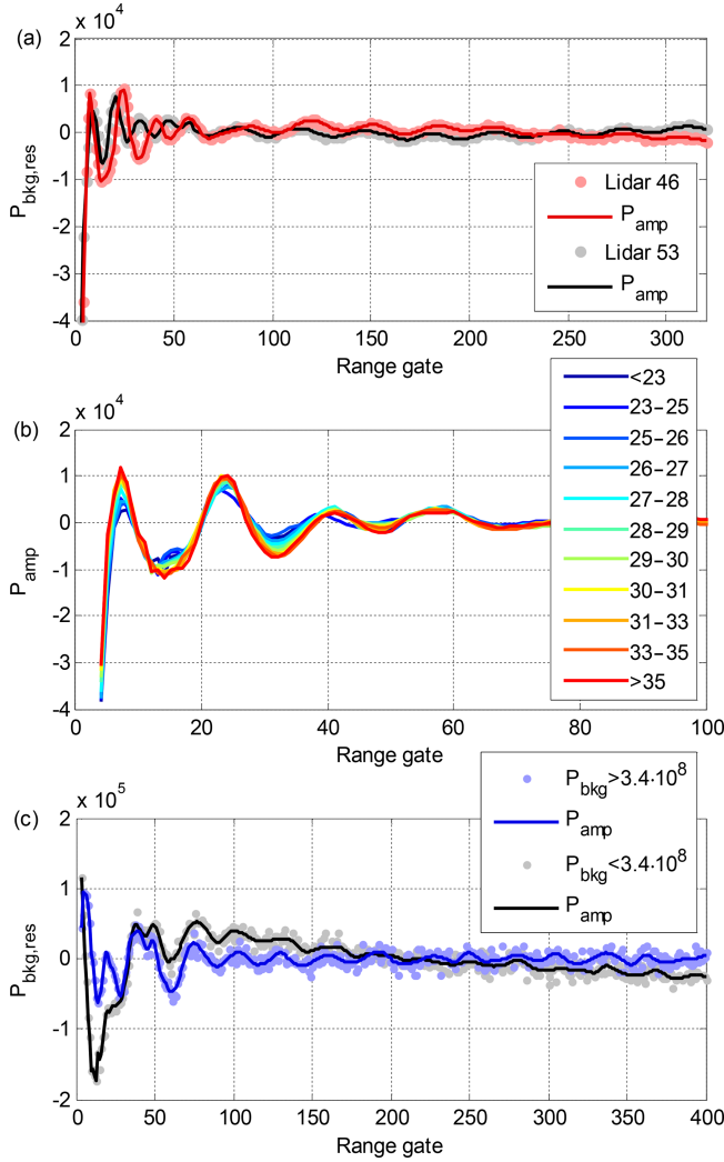
Figure 2. (a) Lidar 46 P_{\text{bkg, res}} averaged from 20 August 2016 to 14 June 2017 (7193 background checks). Lidar 53 P_{\text{bkg, res}} averaged from 1 January 2014 to 30 November 2015 (16 802 background checks). P_{\text{amp}} is plotted for both systems. (b) First 100 range gates of lidar 46 P_{\text{amp}} calculated for different ranges of T . (c) Lidar 146 P_{\text{bkg, res}} averaged from 12 January to 31 May 2018. P_{\text{bkg, res}} is averaged separately for high P_{\text{bkg}} mode (1375 background checks) and for low P_{\text{bkg}} mode (1623 background checks). P_{\text{amp}} is plotted for both modes.
