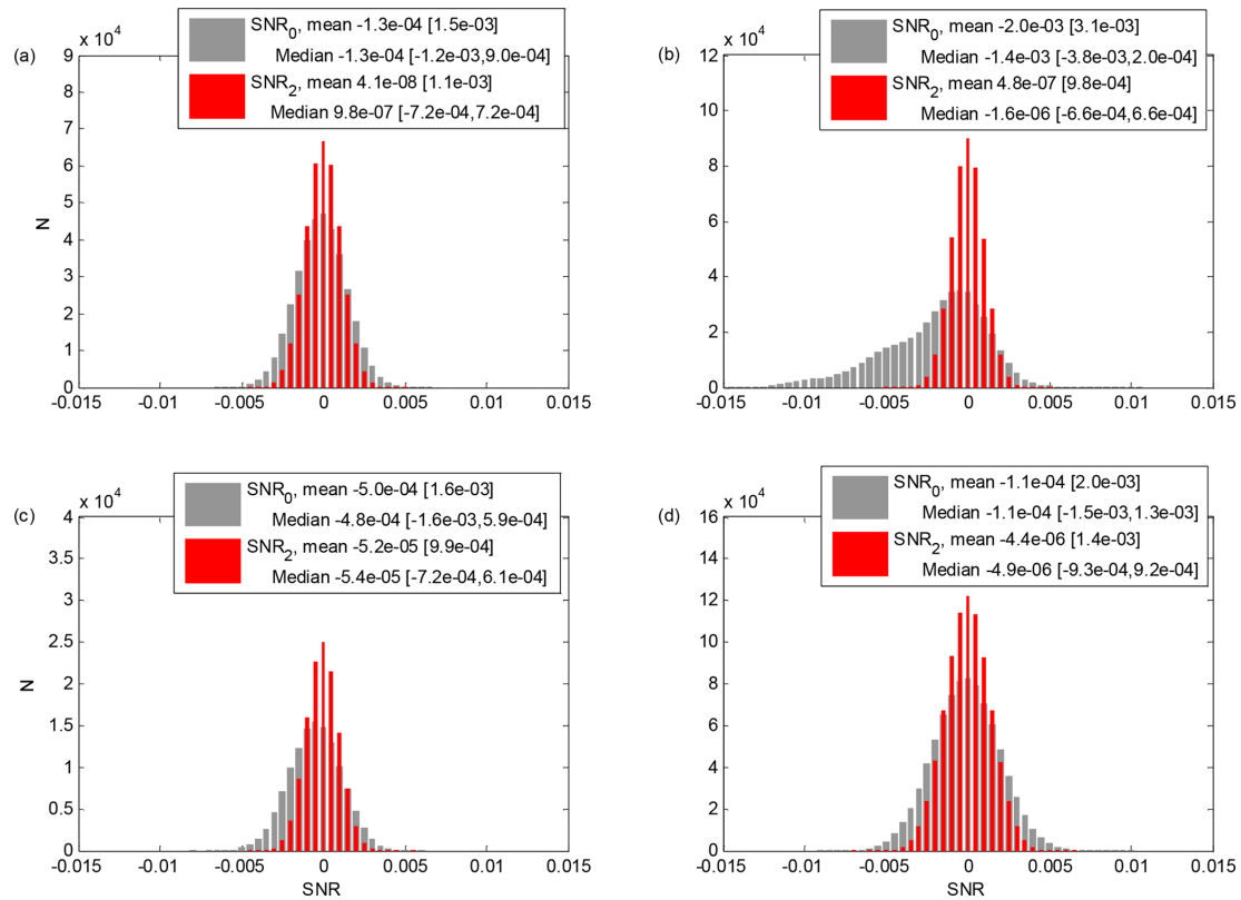
Figure A1. Histograms of SNR 0 and SNR 2 in a cloud- and aerosol-free regime for the four case studies considered in Sect. 4. For each case, mean [standard deviation] and median [25th, 75th percentile] of SNR 0 and SNR 2 are included. (a) Welgegund on 6 September 2016, 00:00–24:00 UTC, 4800–9000 m a.g.l. (b) Kumpula on 1 May 2018, 02:00–24:00 UTC, 6000–12 000 m a.g.l. (c) Kumpula on 6 May 2018, 00:00–12:00 UTC, 4000–7000 m a.g.l. (d) Finokalia on 8 July 2014, 00:00–24:00 UTC, 5000–96 000 m a.g.l.
