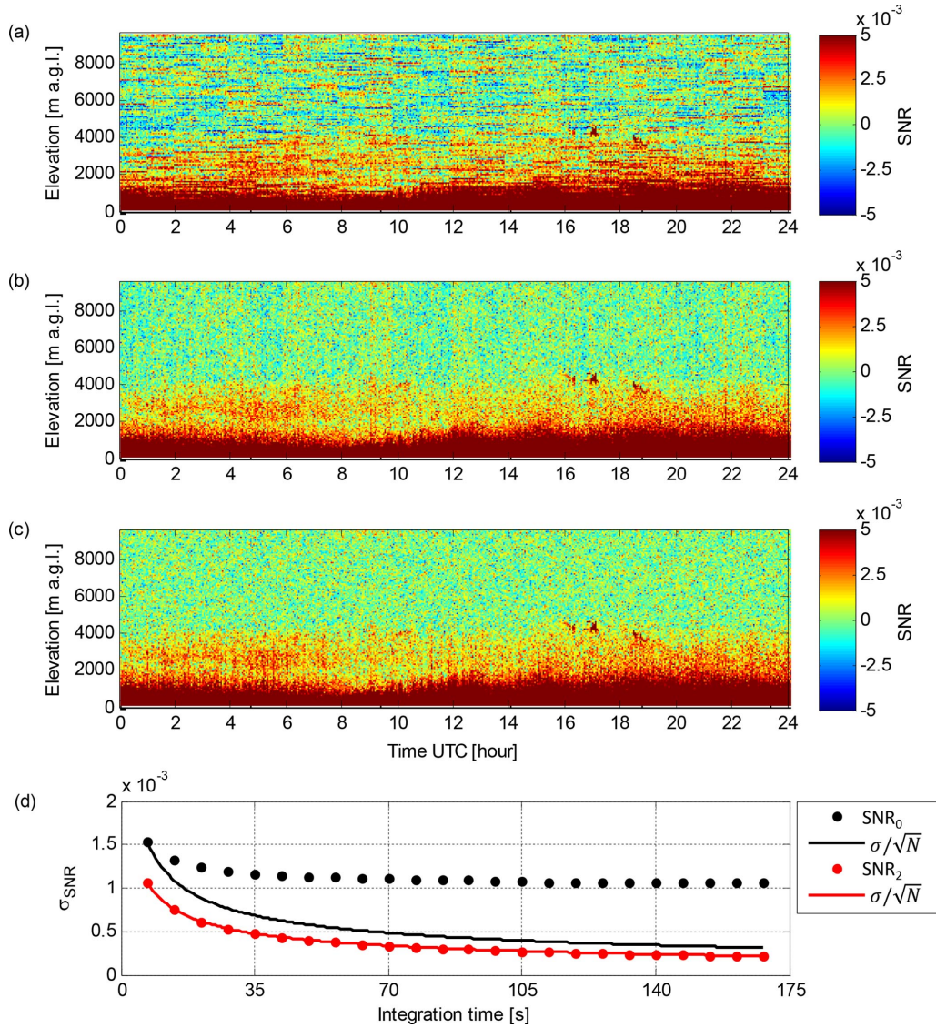
Figure 4. Data from lidar 46 at Welgegund on 6 September 2016. (a) Time series of the SNR 0 profile in vertically pointing mode. (b) Time series of the SNR 1 profile in vertically pointing mode. (c) Time series of the SNR 2 profile in vertically pointing mode. (d) \sigma_{\text{SNR}} as a function of integration time per profile for SNR 0 and SNR 2 for range gates at 4800–9000 m a.g.l. Also \sigma/\sqrt{N} , where \sigma is \sigma_{\text{SNR}} at an integration time of 7 s (original integration time per profile) and N is the number of averaged profiles, is included in (d).
