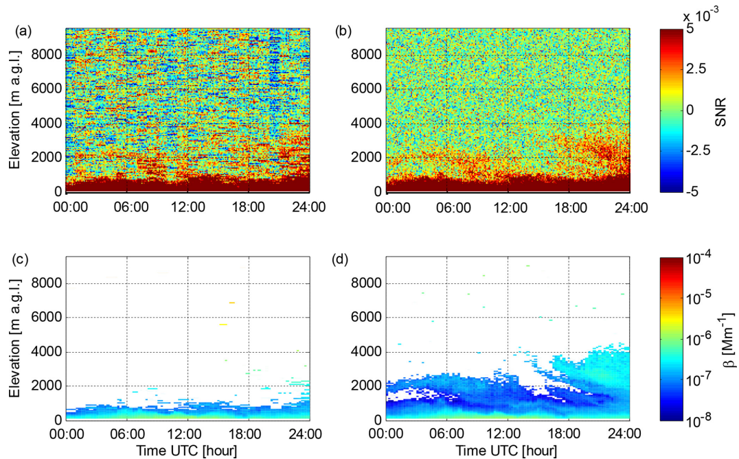
Figure 8. Data from lidar 53 at Finokalia on 8 July 2014. (a) Time series of the \text{SNR}_0 profile in vertically pointing mode. (b) Time series of the \text{SNR}_2 profile in vertically pointing mode. (c) Time series of \beta obtained with 350 s integration time from \text{SNR}_0 ; \beta has been filtered with a threshold of 0.0044 ( 3\sigma ) applied to \text{SNR}_0 . (d) Time series of \beta obtained with 350 s integration time from \text{SNR}_2 ; \beta has been filtered with a threshold of 0.00059 ( 3\sigma ) applied to \text{SNR}_2 .
