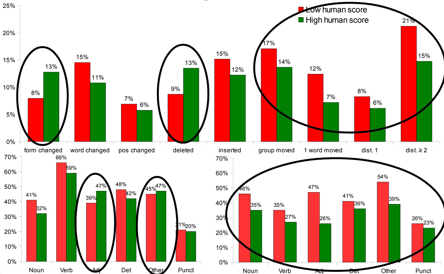
(a) Token edited
