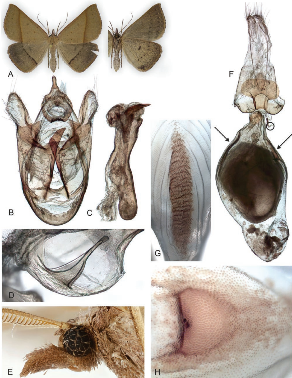
Figure 7. Adults and selected structures of Ecphyas holopsara Turner, 1929. A, adult female, wingspan 35 mm. B, male reproductive organ. C, aedeagus. D, male tympanal organ. E, male head and labial palps. F, female reproductive organ. G, elongated signum. H, roundish signum. Specimen metadata are given in Supporting Information, File S1 .
