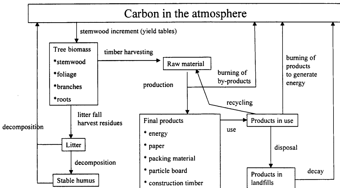
Figure 1. Carbon fluxes/processes (arrows) and carbon stocks (boxes) in a forest ecosystem and its wood products distinguished in CO2FIX.
